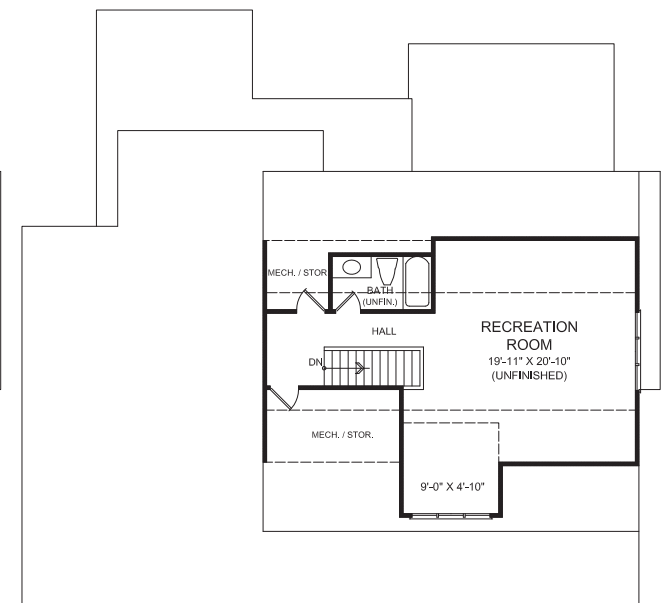
THIRD FLOOR
